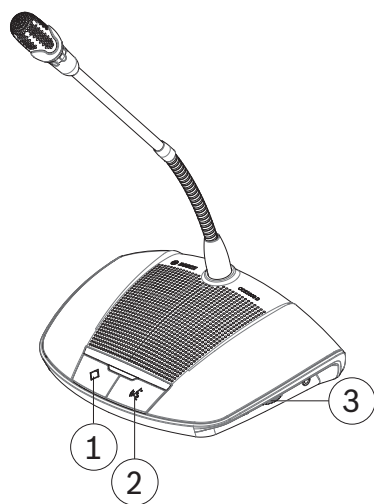
Figure 8.3: Device with chairperson's button fitted
