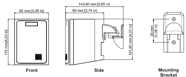
LB6-S-D and mounting bracket
