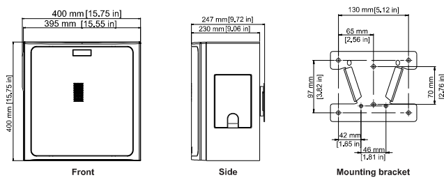
LB6-SW100-D and mounting bracket
